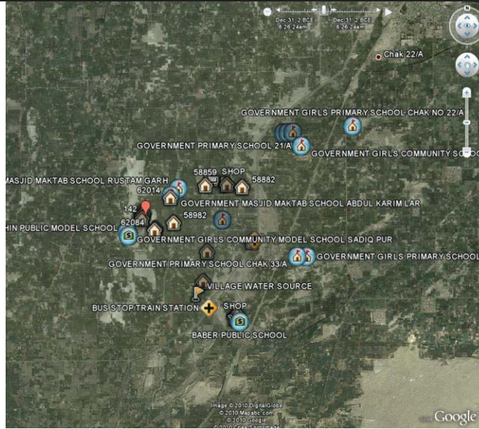
Appendix Figure 1: A Village For Which the Centroid Algorithm Performs Badly
